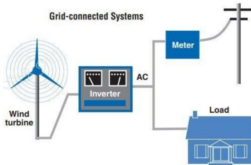
Fig. 5. Wind energy schema (Laboratory, 2007)
