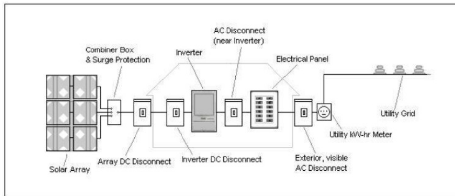
Fig. 4. Work system of solar cell (Roos & Nelson, 2009)
