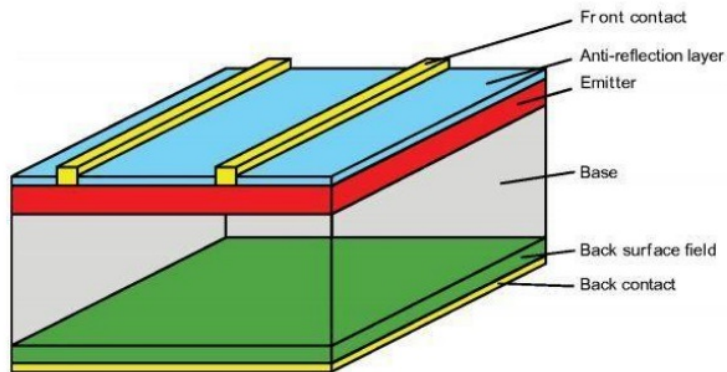
Fig. 3. Section of Solar Cell (Vozel, 2011)
