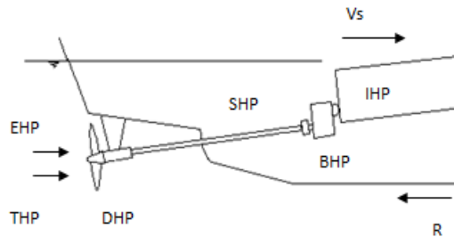
Fig.3. Propulsion System of The Vessel
