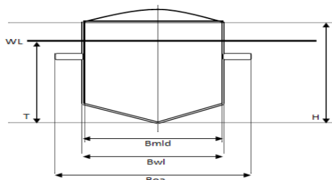
Fig.2. Cross-sectional Shape of the Vessel
