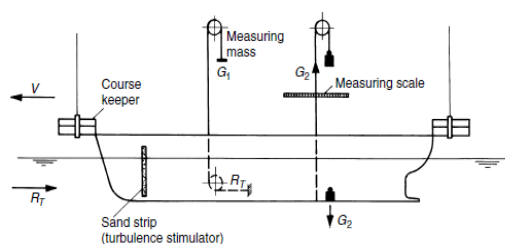
Fig.4. Experimental Set-up For Resistance Test
