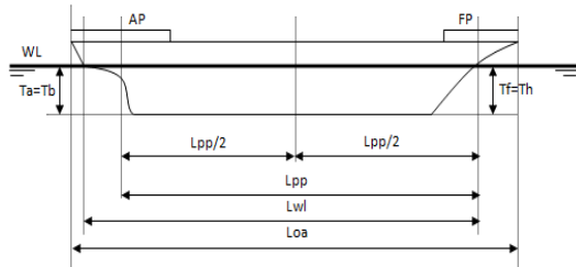
Fig.1. Longitudinal Shape of the Vessel
