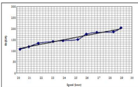
Figure 8: Relationship Between Vessel Speed and Resistance at Draft T : 1.50 and Draft T : 1.65
