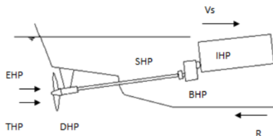
Figure 3: Propulsion System of The Vessel
