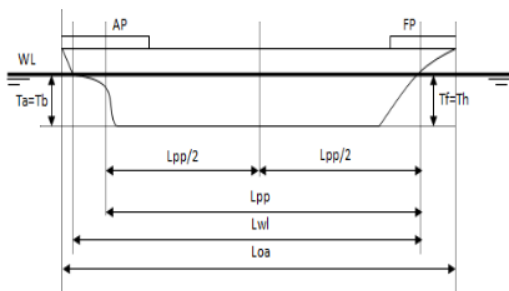
Figure 1: Longitudinal Shape of The Vessel
