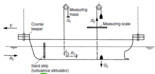
Figure 4: Experimental Set-up For Resistance Test
