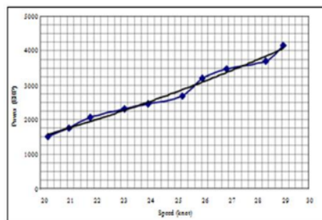
Figure 9: Relationship between Speed and Ship EHP at Draft T : 1.50 and Draft T : 1.65
