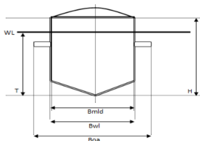
Figure 2: Cross-sectional Shape of The Vessel
