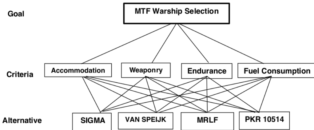
Figure 1. Hierarchy Diagram
